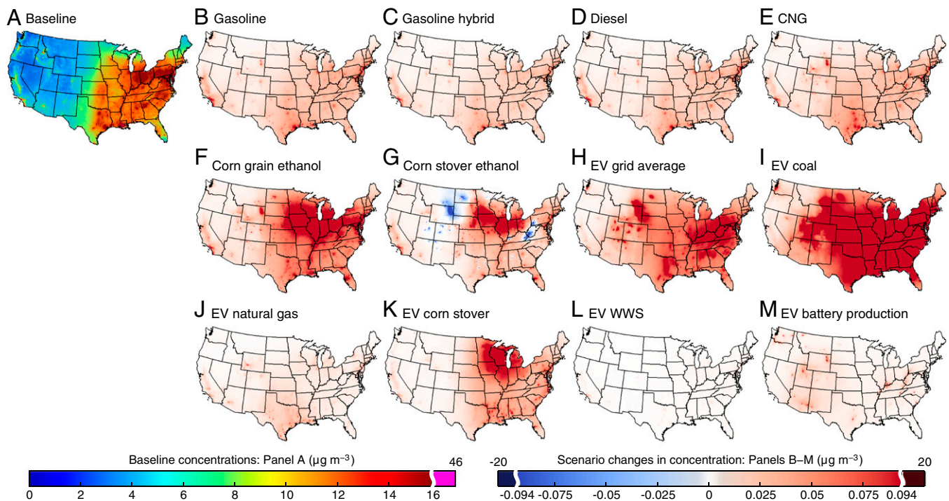
Fig. 1. Annual average PM 2.5 concentrations. (A) Year 2005 baseline modeled concentrations. (B–L) Increase in concentration above the baseline attributable to replacement of 10% of year 2020 vehicle use with the given technology. (M) Increase in concentration attributable to EV battery manufacturing. Color scales contain a discontinuity at the 99th percentile of emissions. Abbreviations: CNG, compressed natural gas vehicle; EV, electric vehicle; WWS, wind, water, or solar. Analogous plots for O 3 are in Fig. S1.
